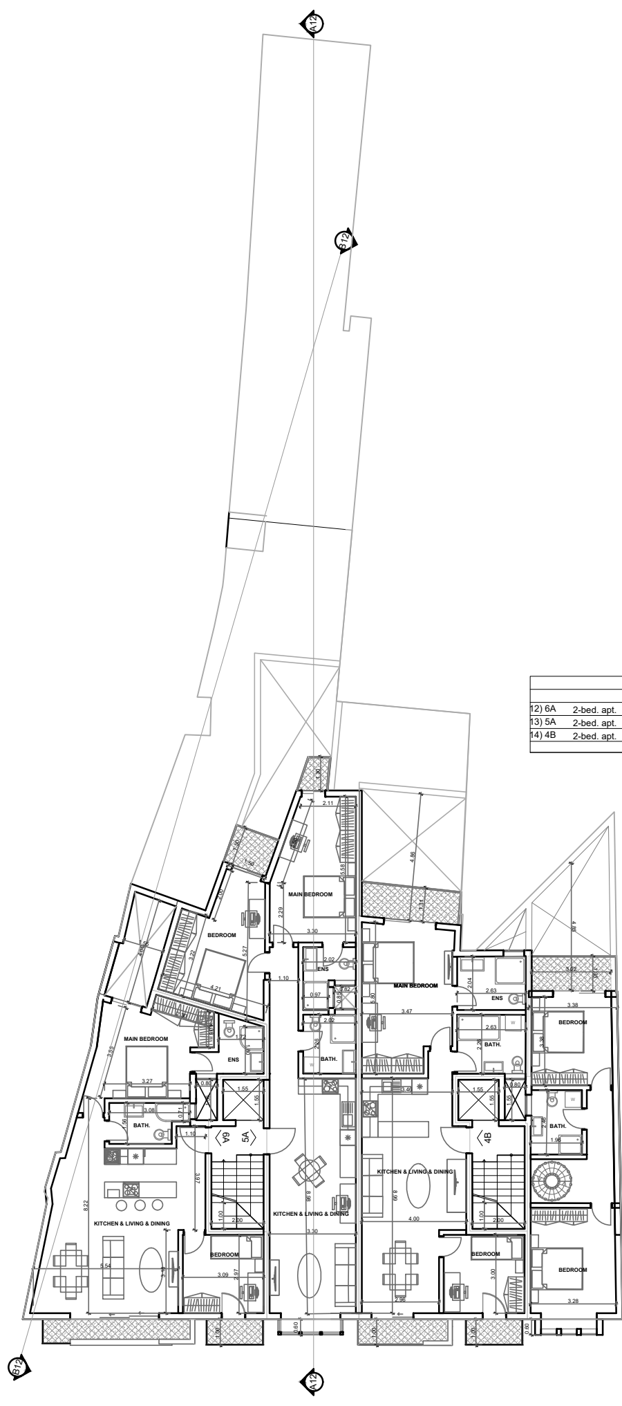
PROPOSED 3RD FLOOR LEVEL
